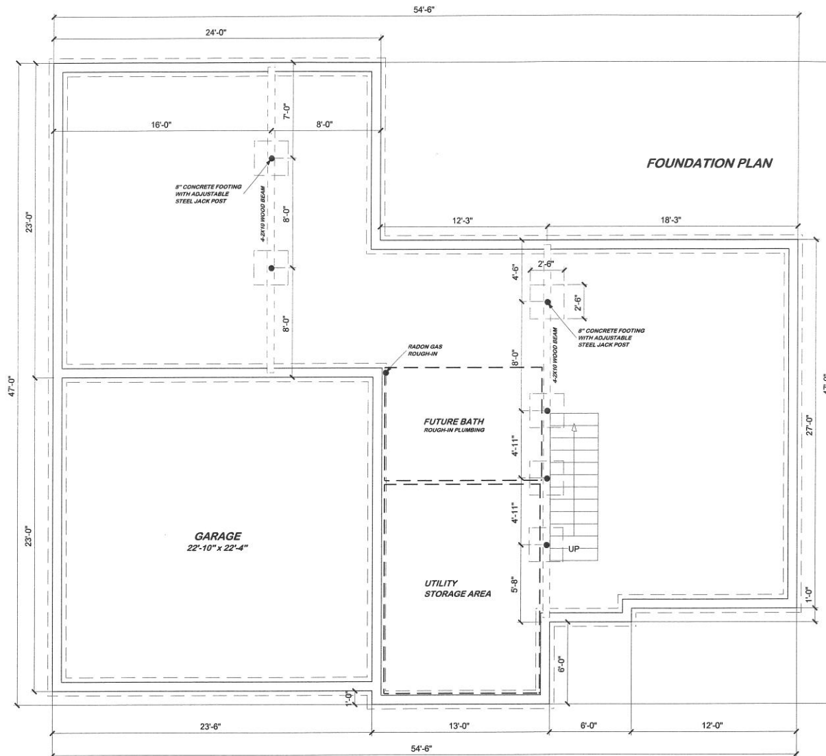
Foundation Plan
